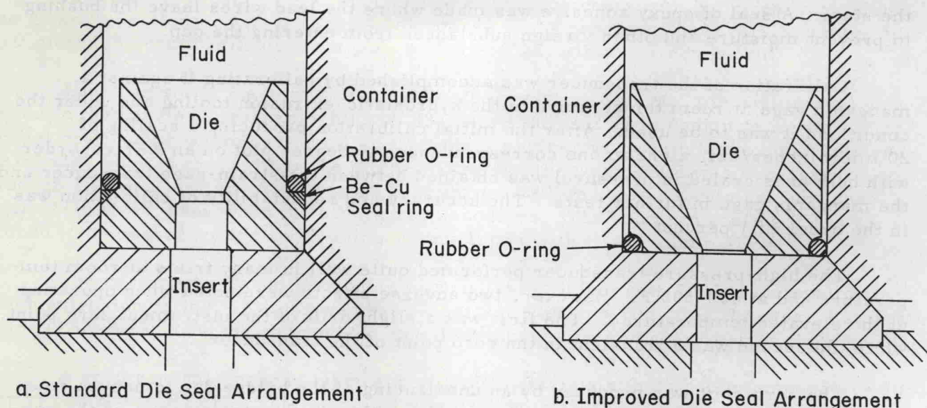
FIGURE 9. DIE SEAL ARRANGEMENTS EVALUATED IN HYDROSTATIC EXTRUSION
